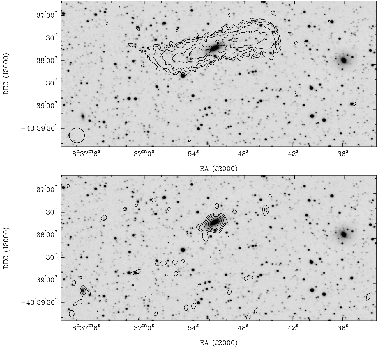
Figure 3. Top: H I distribution of HIZOA J0836-43 (contours) at a resolution of 20'' overlaid onto the AAT K_s -band image (greyscale). The contour levels are the same as in Fig. 2 (bottom left). Bottom: 20-cm radio continuum image of HIZOA J0836-43 (contours) overlaid onto the same K -band image. The contour levels are -0.26, 0.26, 0.52, 1.04, 2.08 , and 4.16 \text{ mJy beam}^{-1} ; the synthesized beam is 8.7'' \times 6.5'' . The displayed region was chosen to also include the two neighbouring galaxies, one of which is detected in the radio continuum with an H I flux density of \sim 1 \text{ mJy} .
