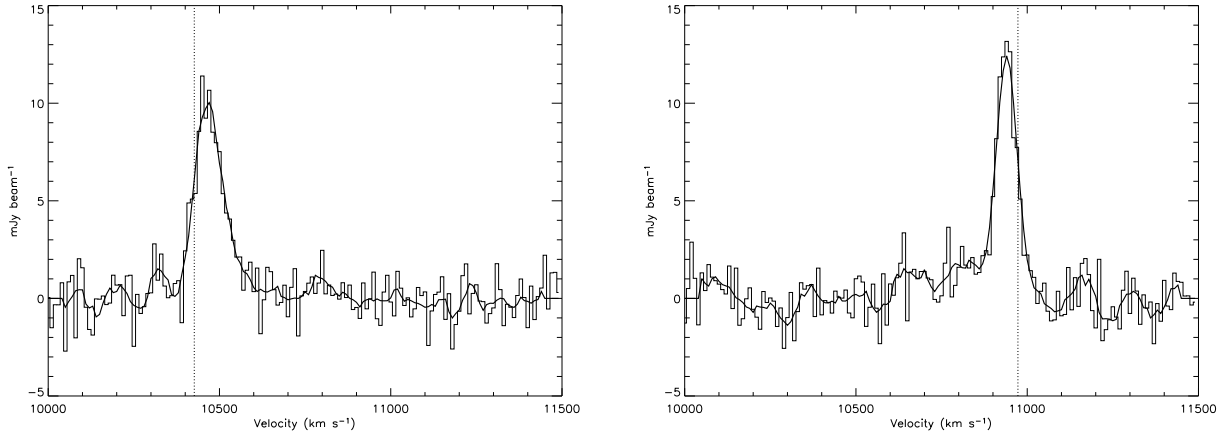
Figure 6. Sample H I velocity profiles of HIZOA J0836-43 obtained from the major-axis pv -diagram at offsets of -0.9' and 1.0' . Dotted lines represent the rotation velocity measured for each slice. Both the unsmoothed and the Savitzky-Golay smoothed profiles are shown for comparison.
