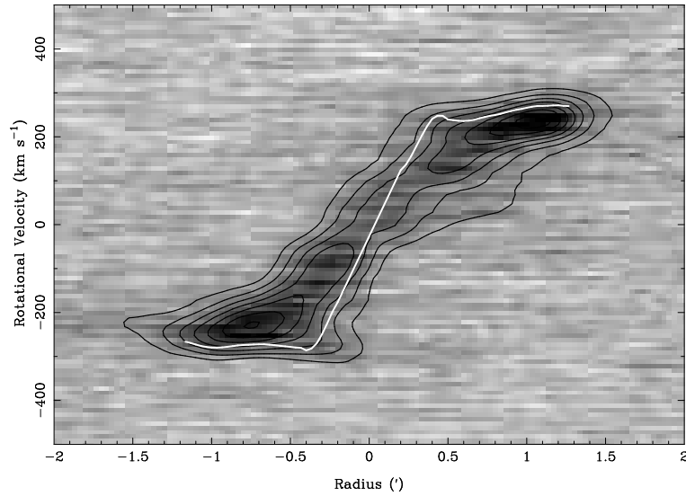
Figure 5. H I position-velocity ( pv ) diagram along the major axis ( PA = 285^\circ ) of HIZOA J0836-43 using the combined H I data set with an angular resolution of 20'' . The white line gives the H I rotation curve as shown in Fig. 8. Contours represent intensity levels of 2-8\sigma , where \sigma = 1.14 \text{ mJy beam}^{-1} , and are measured after smoothing the pv -diagram by a Gaussian kernel of width 2.
