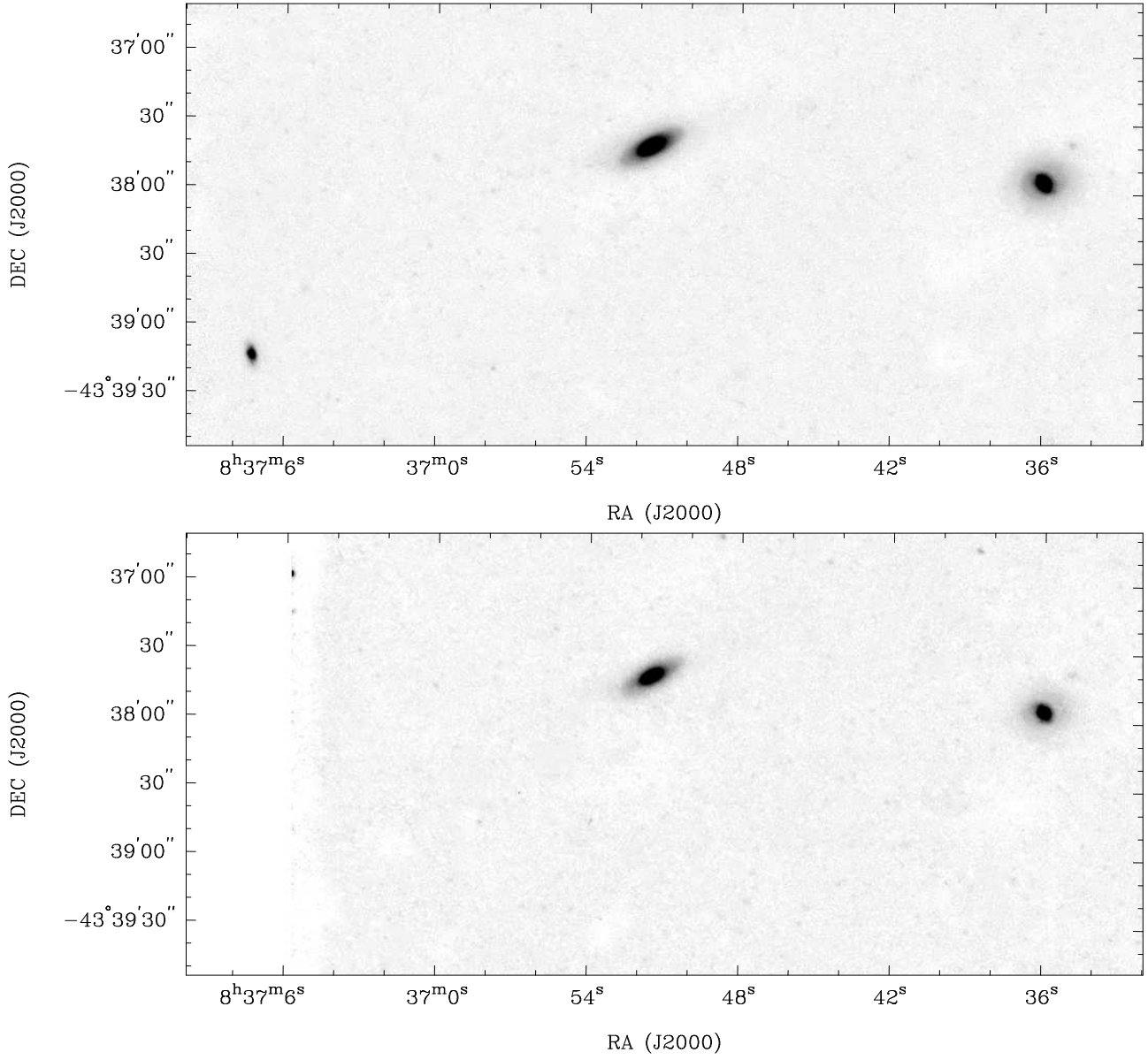
Figure 8. Star-subtracted AAT K_s -band image (top) and H -band image (bottom) of HIZOA J0836-43 and neighbouring galaxies.
