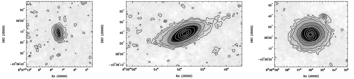
Figure 9. Star-subtracted AAT K_s -band images of 2MASX J08370723-4339137 (left), HIZOA J0836-43 (middle) and 2MASX J08363600-4337556 (right). The contour levels are 30, 80, 160, 320, 640, 1280, 2560, 5120, and 10240 units. The images were convolved with a 1''.5 Gaussian.
