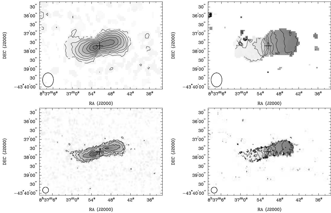
Figure 2. H I distribution (left) and mean H I velocity field (right) of the galaxy HIZOA J0836–43. Contour levels are 0.1, 0.3, 0.6, 1, 1.5, 2.0, 2.5, and 3.0 Jy beam −1 km s −1 (top left; 1 Jy beam −1 km s −1 equals an H I column density of 6.8 \times 10^{20} cm −2 ), 0.1, 0.2, 0.4, 0.8, 1.2, and 1.6 Jy beam −1 km s −1 (bottom left; 1 Jy beam −1 km s −1 equals an H I column density of 3.0 \times 10^{21} cm −2 ), and 10450 to 10950 km s −1 in steps of 50 km s −1 (right). The synthesized beam is shown in the bottom left corner of each frame (47.5'' × 36.7'' on the top, and 20'' on the bottom). The cross marks the galaxy centre as determined from the 20-cm radio continuum (see Table 2).
